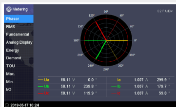
Phasor Diagram
