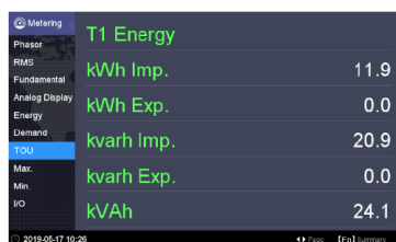
Large Character TOU Energy Display
